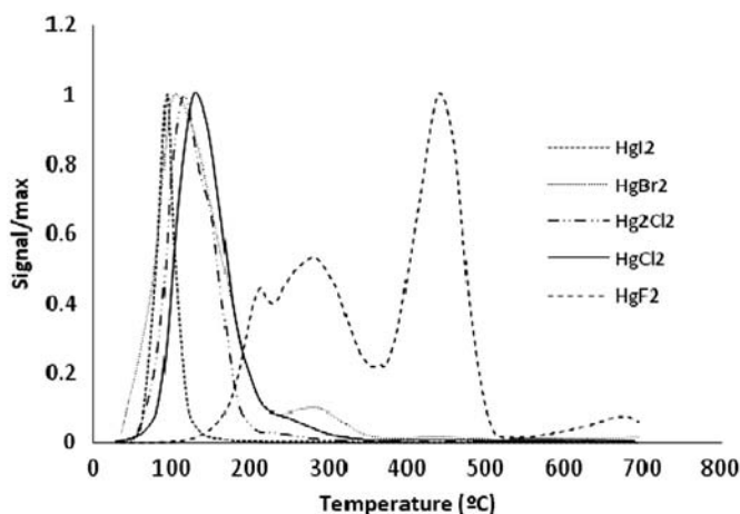
Fig. 1. Thermal-desorption profiles of the Hg-halides.
