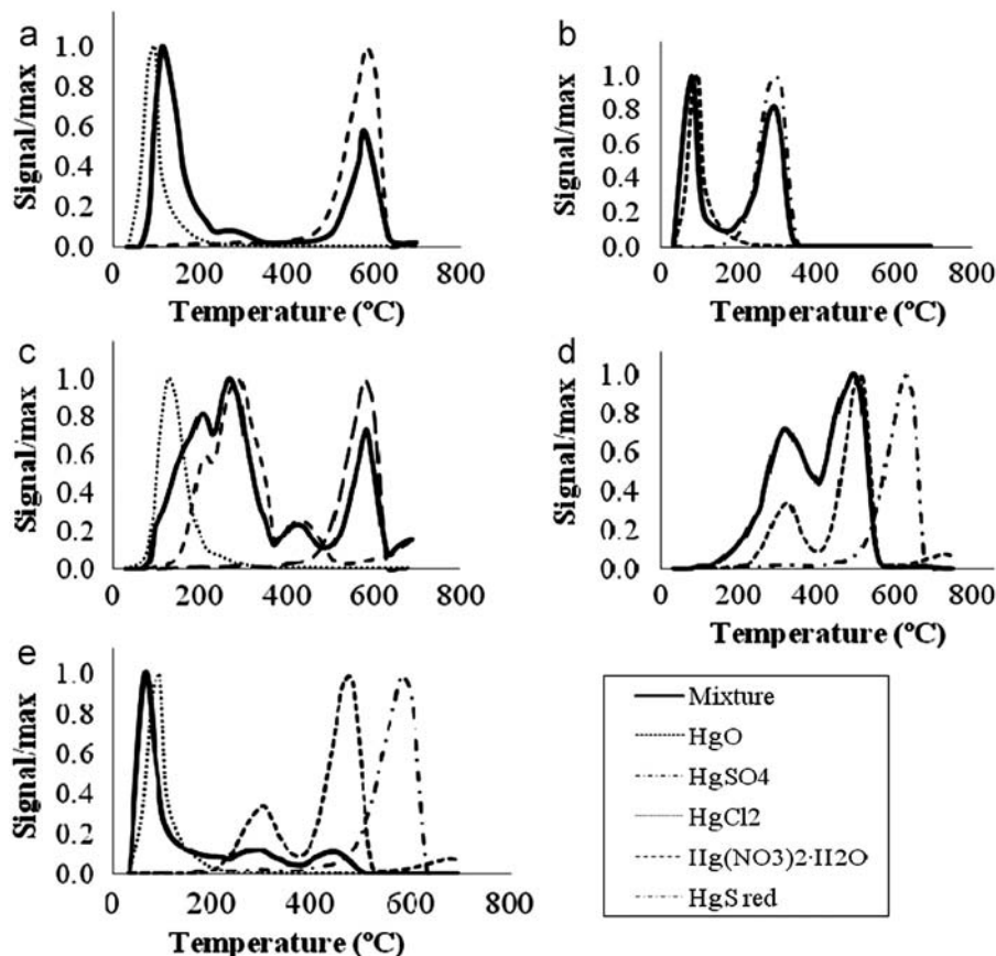
Fig. 6. Thermal-desorption profiles of the mixtures: (a) HgCl 2 :HgSO 4 (1:1); (b) HgCl 2 :HgS red (1:1); (c) HgCl 2 :Hg(NO 3 ) 2 · H 2 O: HgSO 4 (1:1:1); (d) HgO red: HgSO 4 (1:1) and (e) HgCl 2 :HgO red: HgSO 4 (1:1:1).
