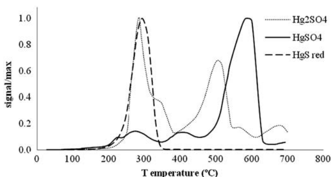
Fig. 3. Thermal-desorption profiles of the S-containing mercury compounds.
