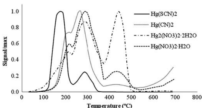
Fig. 4. Thermal-desorption profiles of the N-containing mercury compounds.
