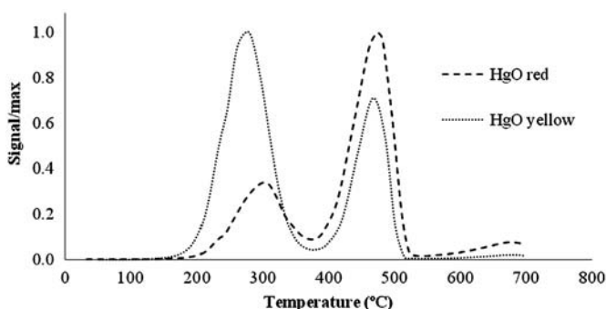
Fig. 2. Thermal-desorption profiles of the mercury oxides.
