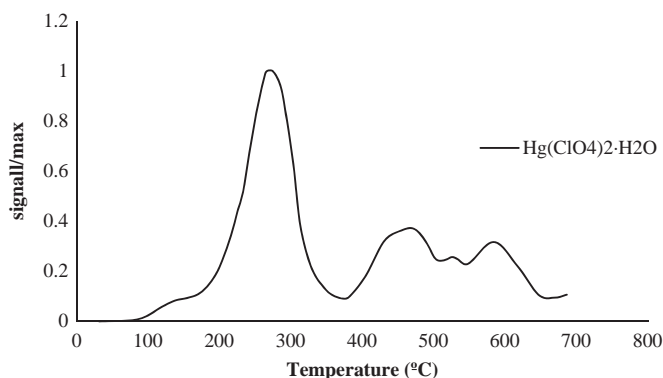
Fig. 5. Thermal-desorption profiles of mercury(II) perchlorate hydrate.
